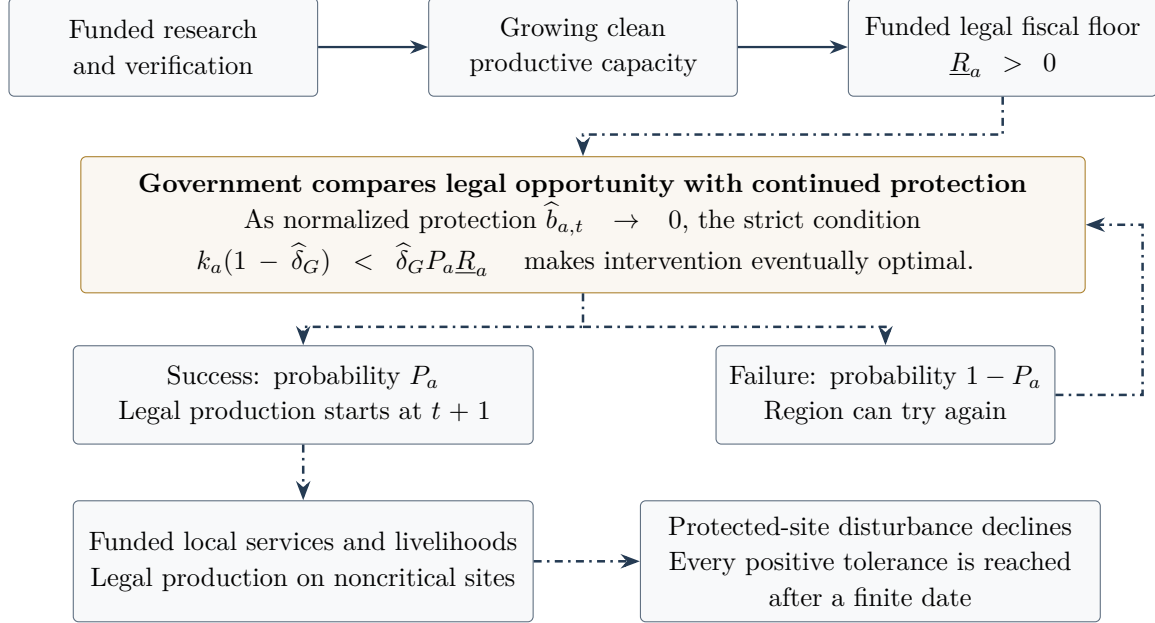
Figure 6: Scarcity and the conditional route to conservation. Panel A holds dirty expenditure and clean supply fixed: less aggregate illegal extraction can coexist with higher surviving-region rents. In panel B, navy dash-dot arrows show the conditional path and repeated attempts; the gold frame highlights the fiscal comparison. Intervention becomes optimal after a finite date under the stated conditions, while protected-site disturbance declines through repeated attempts. Some ungoverned mass can remain at every finite date, and fixed dirty cores remain productive. Historical origin and liabilities persist; irreversible losses remain subject to the cumulative-disturbance budget.
