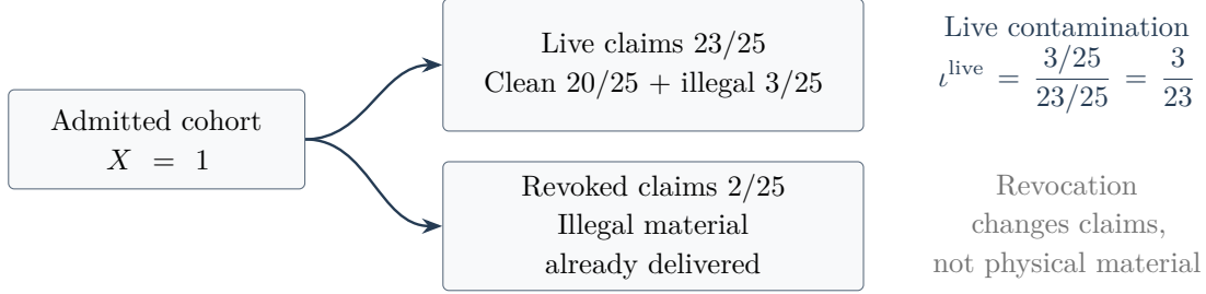
Figure 4: Deliveries and claim status in Example 6.2. Panel A conserves mineral: total extraction and total delivery both equal 9/5 ; panel B follows the admitted unit through scrutiny, with 23/25 + 2/25 = 1 .
