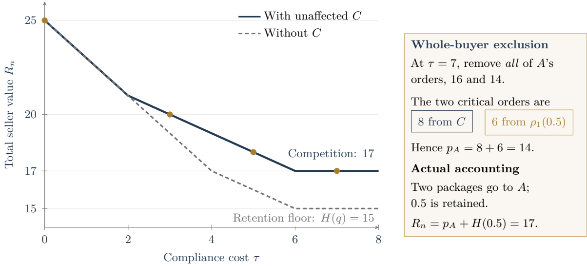
Figure 3: Two buffers for VCG seller value at fixed inventory. Dots mark the with- C observations in Table 1.
